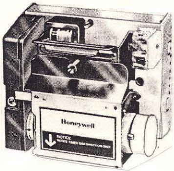
R4140G,L,M Controls
